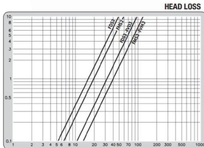
Results obtained in our facilities with approved measuring instruments, using clean water as a fluid for assessment with 190µm red disc Lama.
